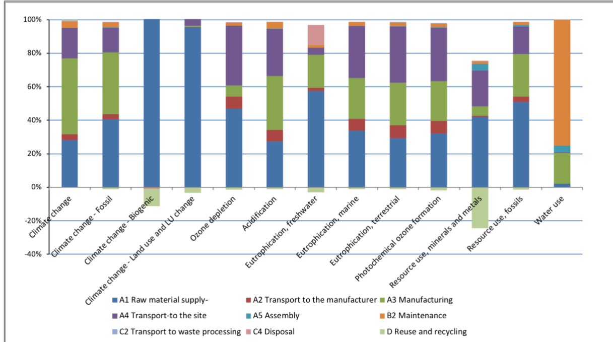
Figure 1 Contribution analysis of environmental impact results using EN 15804+A2 method
